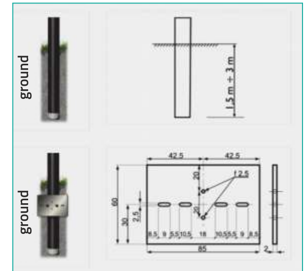
Armament based on the album LnniS Volume 1 of the STELEN 2011 publishing house.
